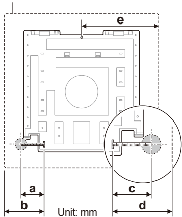
Framework of Indoor Unit
